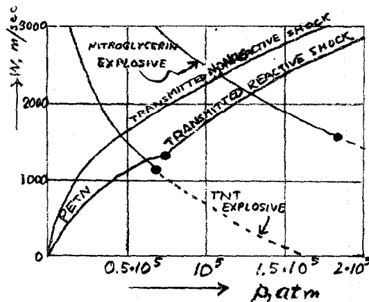
Fig 2 PETN at 1.0 g/cm³ primed by two explosives • = CJ-points
